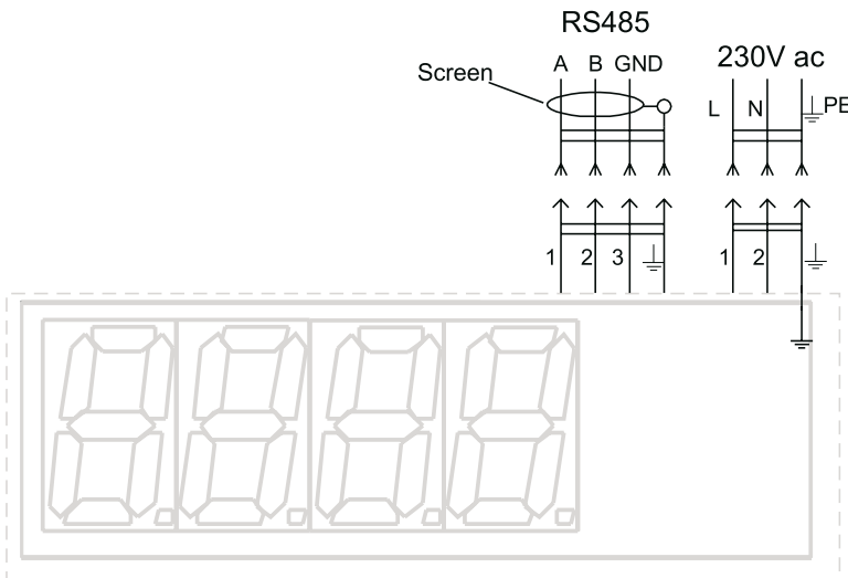
Fig.6. Electrical connections
