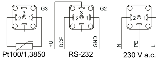
Fig. 9 Description of sockets to connect the mains and application elements: temperature and time for DN3
